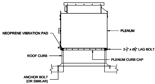
Figure-3. Plenum to Curb Attachment
